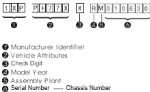
Figure 22 Vehicle Identification Number (VIN)
